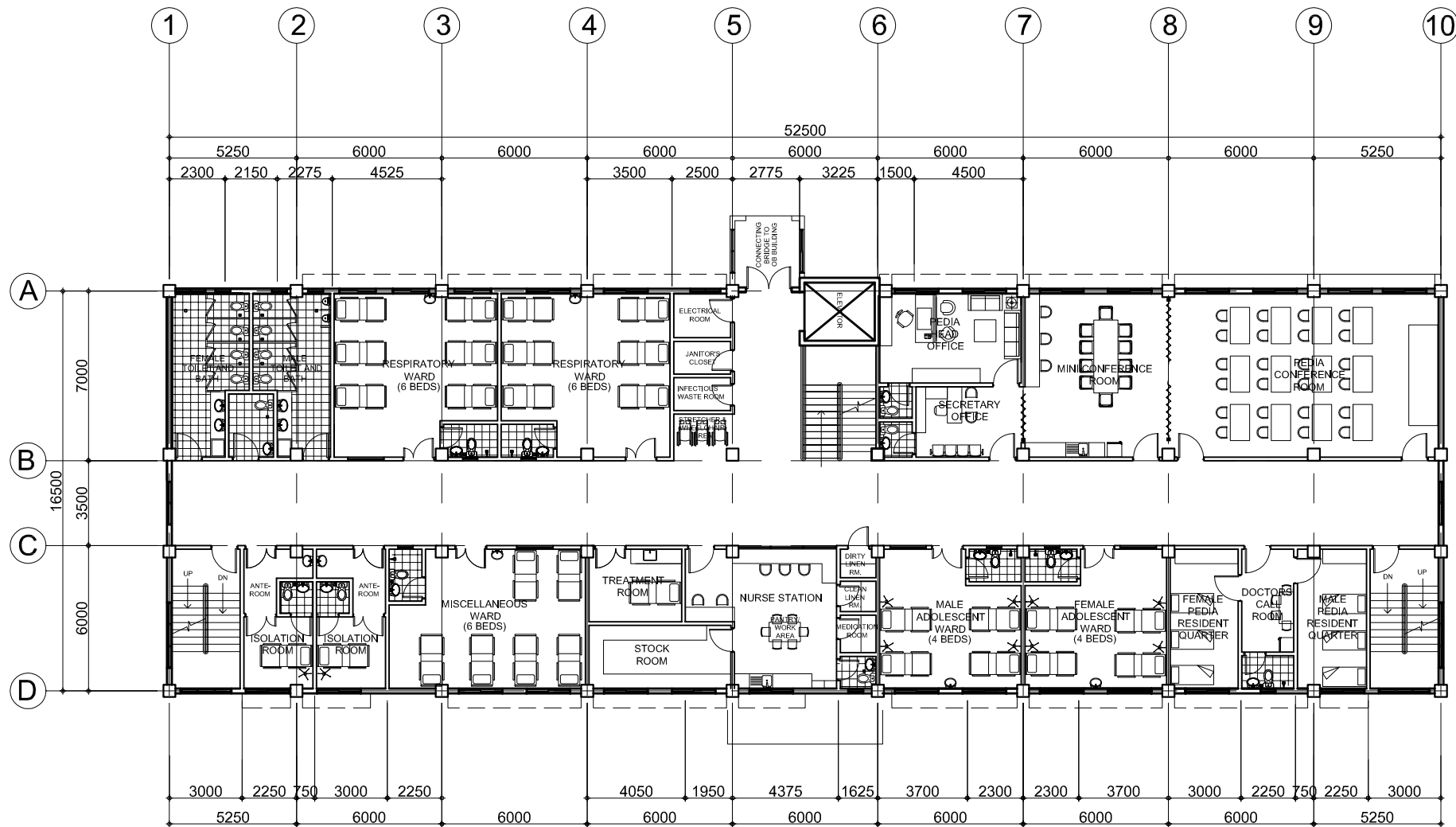
SECOND FLOOR PLAN (ASBULT) SCALE 1:100 mts.
