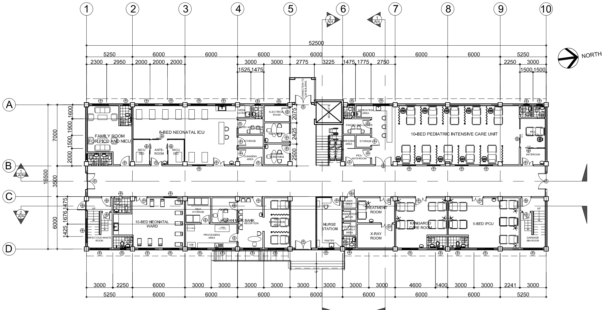
GROUND FLOOR PLAN (ASBUILT) SCALE 1:100 mts.
