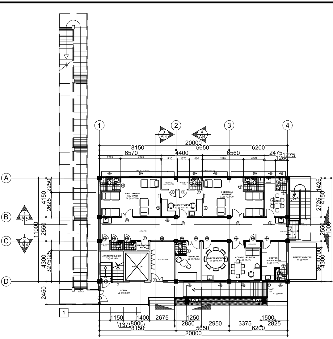
GROUND FLOOR PLAN (ACUTE STROKE UNIT) ASBULT
