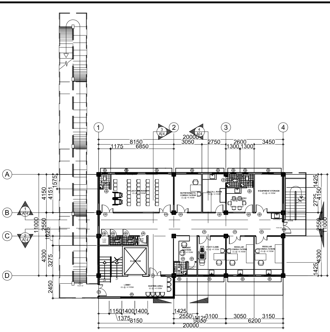
SECOND FLOOR PLAN (DIABETES CONTROL CENTER) ASBULT
