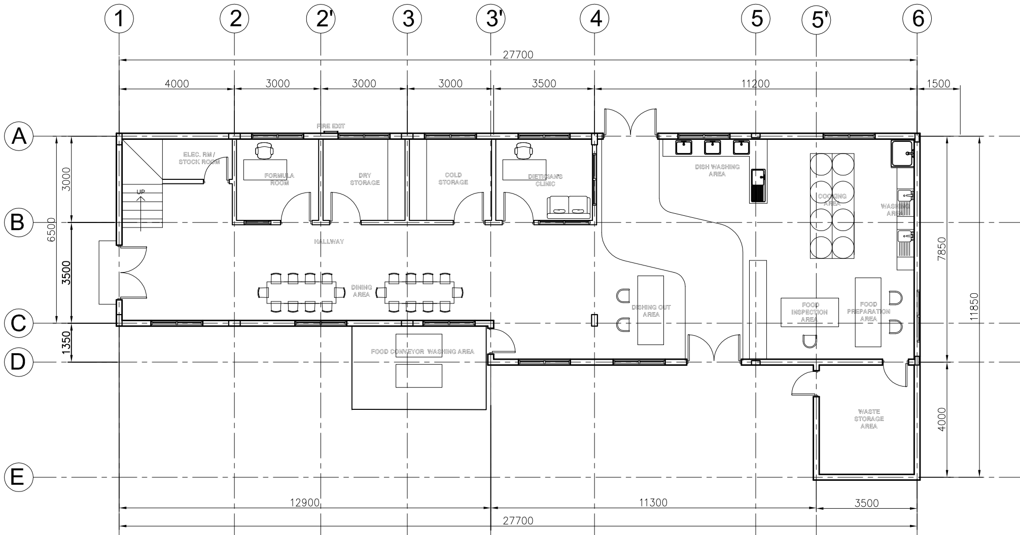
1 A 2 GROUND FLOOR PLAN SCALE 1:100M
